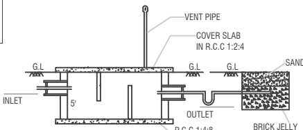
SECTION-AB
