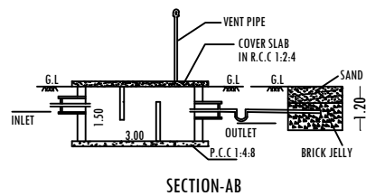
SECTION-AB
