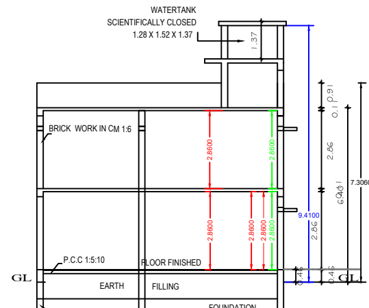
SECTION "A-B"
