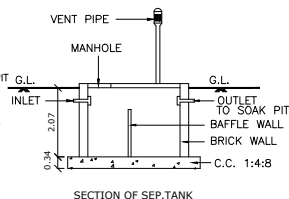
SECTION OF SEPT.TANK
