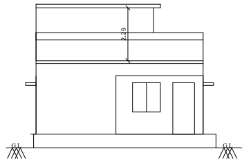
ELEVATION 7.23
