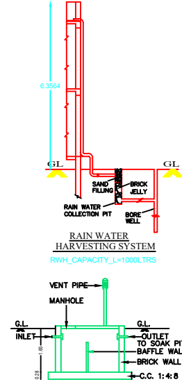
SECTION OF SEP.TANK
