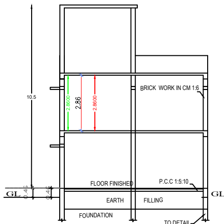
SECTION "A-B"
