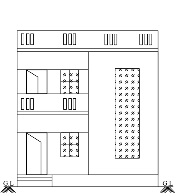
FRONT ELEVATION
