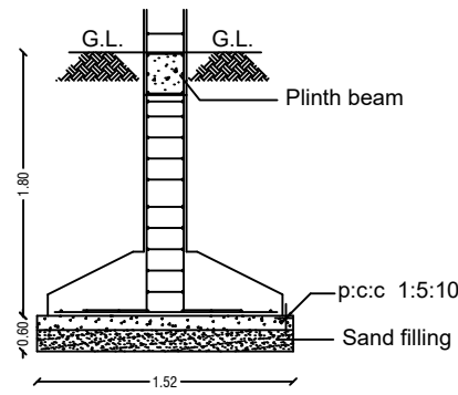
FOUNDATION DETAILS
