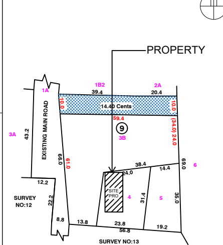
LOCATION PLAN
