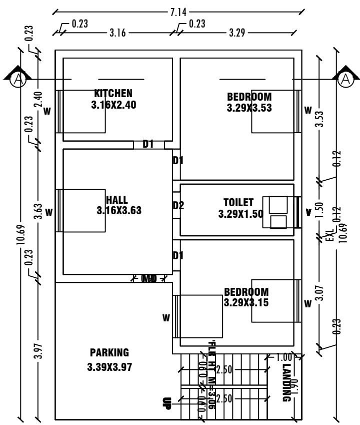
LOOR PLAN :1:100
