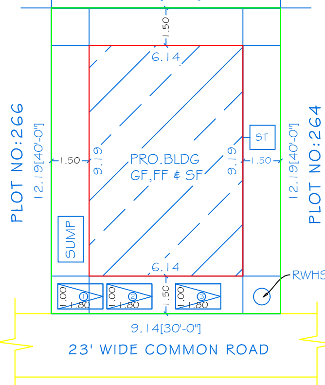
SITE PLAN
