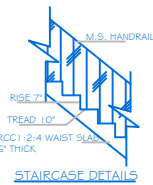
STAIRCASE DETAILS
