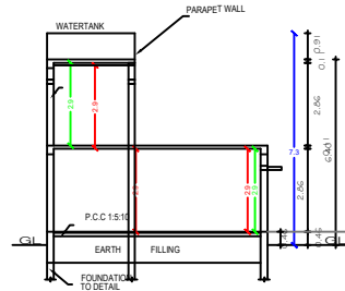
SECTION "A-B"
