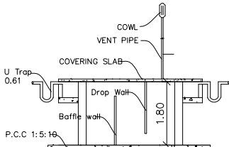
SECTION ON JS
