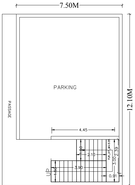
STILT FLOOR PLAN
