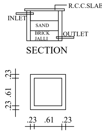
PLAN OF RAIN WATER HARVESTING PIT [SIZE: 2' X2' X 3']
