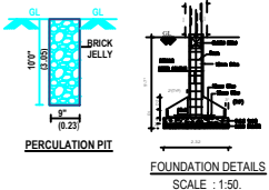
FOUNDATION DETAILS
