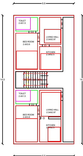
PRO. FIRST FLOOR PLAN.
