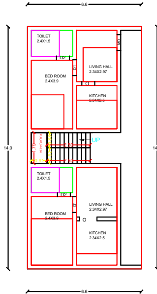
PRO. SECOND FLOOR PLAN.
