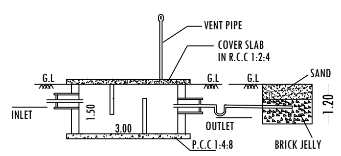
SECTION-AB
