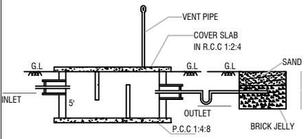
SECTION-AB
