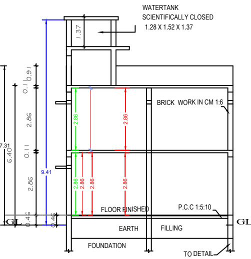
SECTION "A-B"
