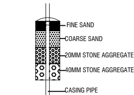
DETAILS OF RAIN WATER HARVESTING STRUCTURES
