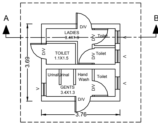
TOILET BLOCK PLAN
