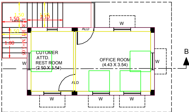
PLAN FIRST FLOOR
