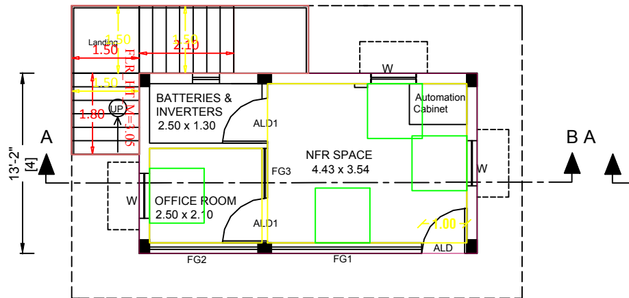
PLAN GROUND FLOOR
