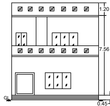
ELEVATION BY NORTH
