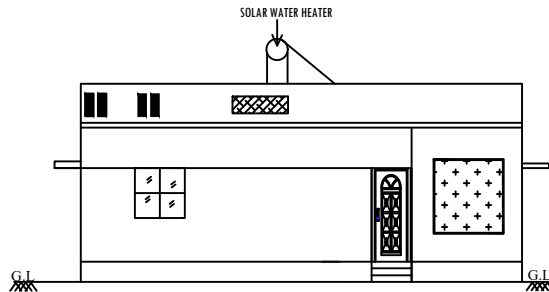
ELEVATION PLAN
