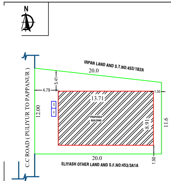
SITE PLAN
