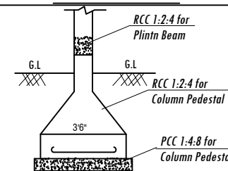
Typical Cross-Section
