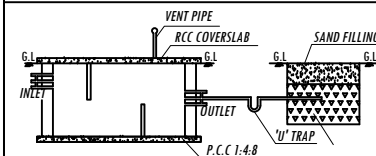
SECTION DETAILS
