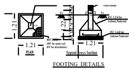
FOOTING DETAILS
