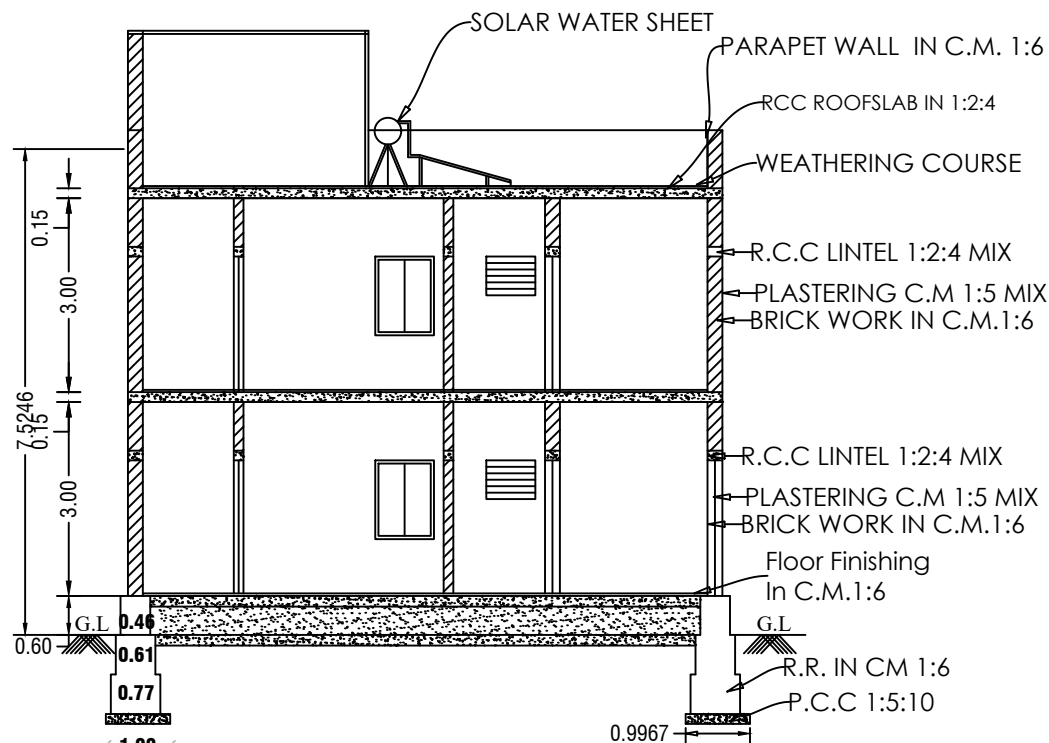
Section On-"AB"
