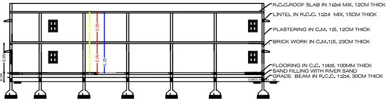
SECTION "AA"
