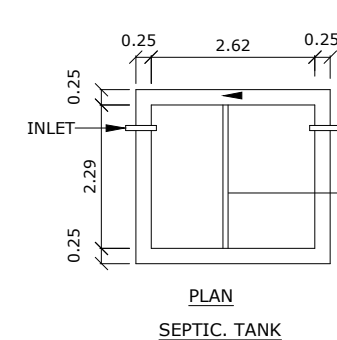
SEPTIC. TANK
