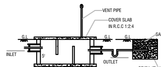
SECTION-AB
