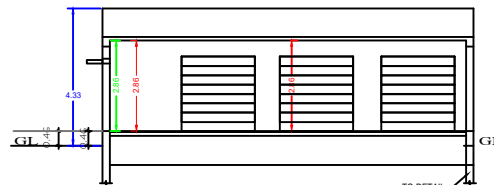
SECTION "A-B"
