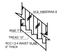
STAIRCASE DETAILS SCALE- 1:20
