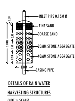
DETAILS OF RAIN WATER HARVESTING STRUCTURES
