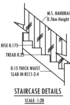
STAIRCASE DETAILS
