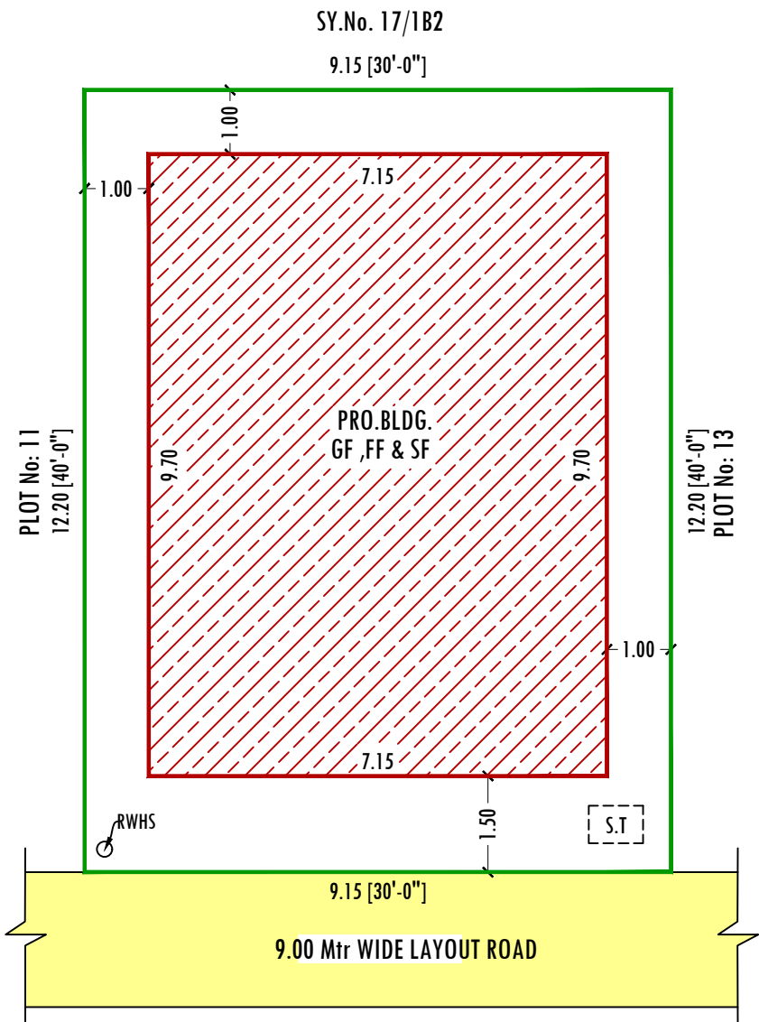
SITE PLAN
