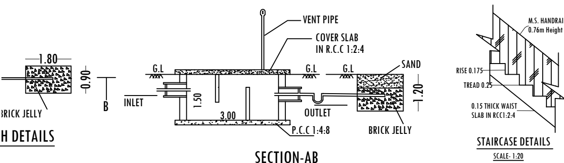
SECTION-AB
