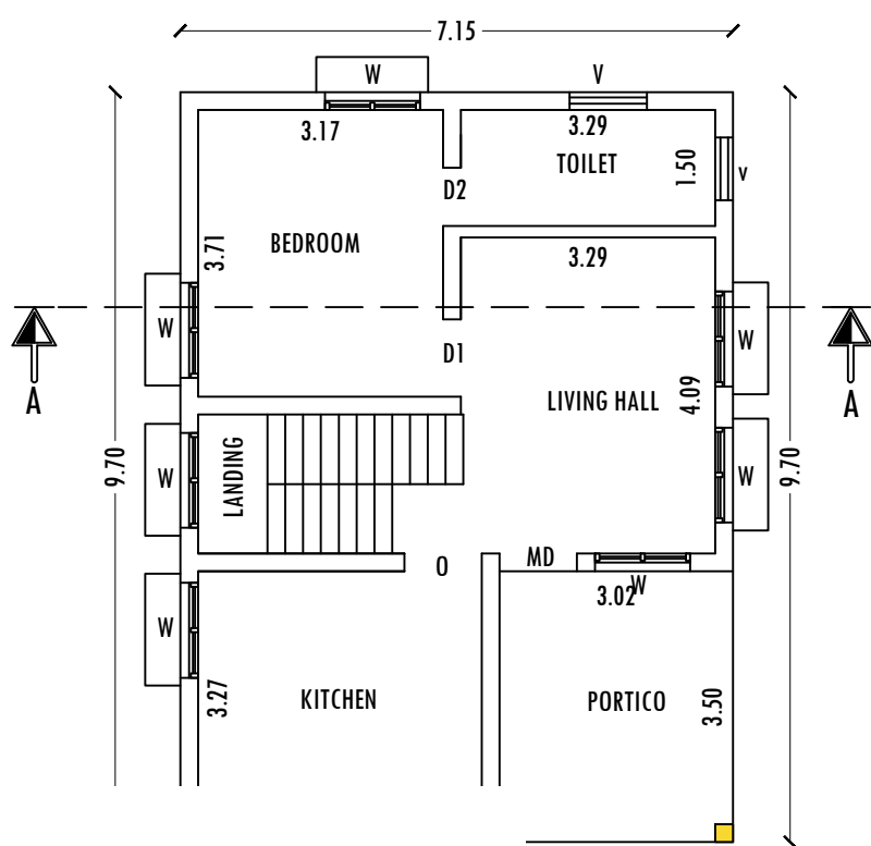
OR PLAN
