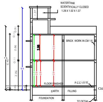
SECTION "A-B"
