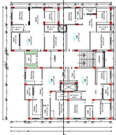
TYPICAL FLOOR PLAN OF FIRST, SECOND & THIRD FLOORS
