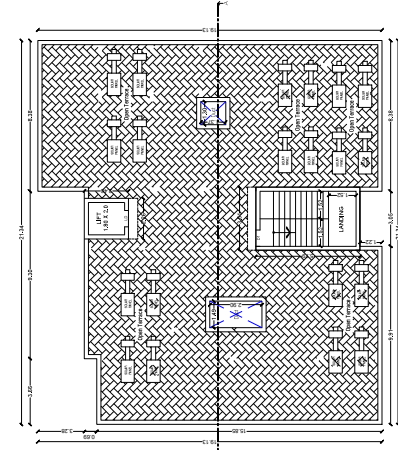
HEAD ROOM / TERRACE FLOOR PLAN
