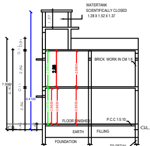
SECTION "A-B"
