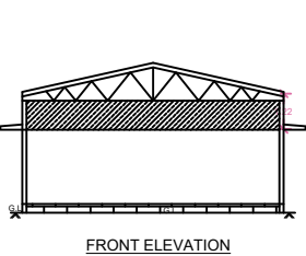
FRONT ELEVATION
