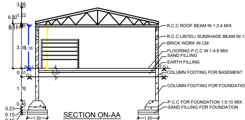
SECTION ON-AA
