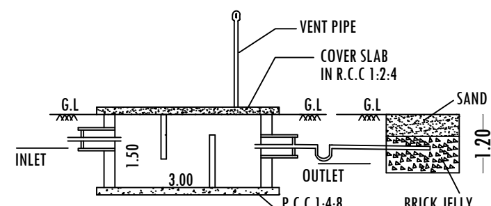
SECTION-AB
