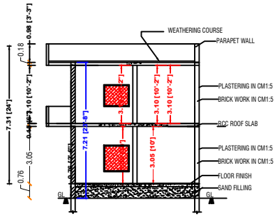
SECTION - AB'
