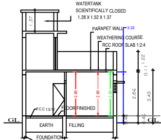
SECTION "A-B"
