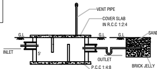
SECTION-AB
