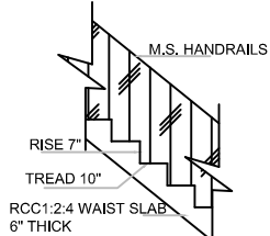
STAIRCASE DETAILS SCALE- 1:20
