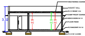
SECTION "A-B"
