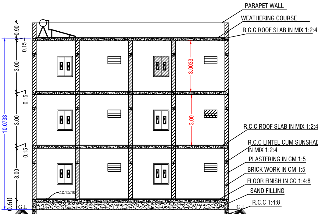
SECTION ON-AA'
