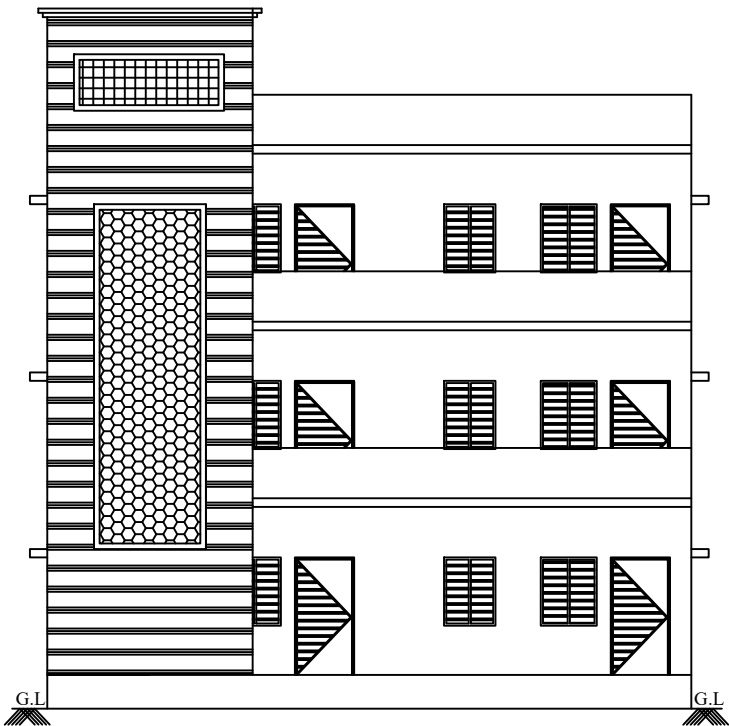
ELEVATION PLAN
