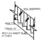
STAIRCASE DETAILS SCALE: 1/20
