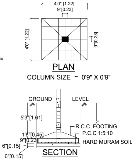
FOUNDATION DETAILS
