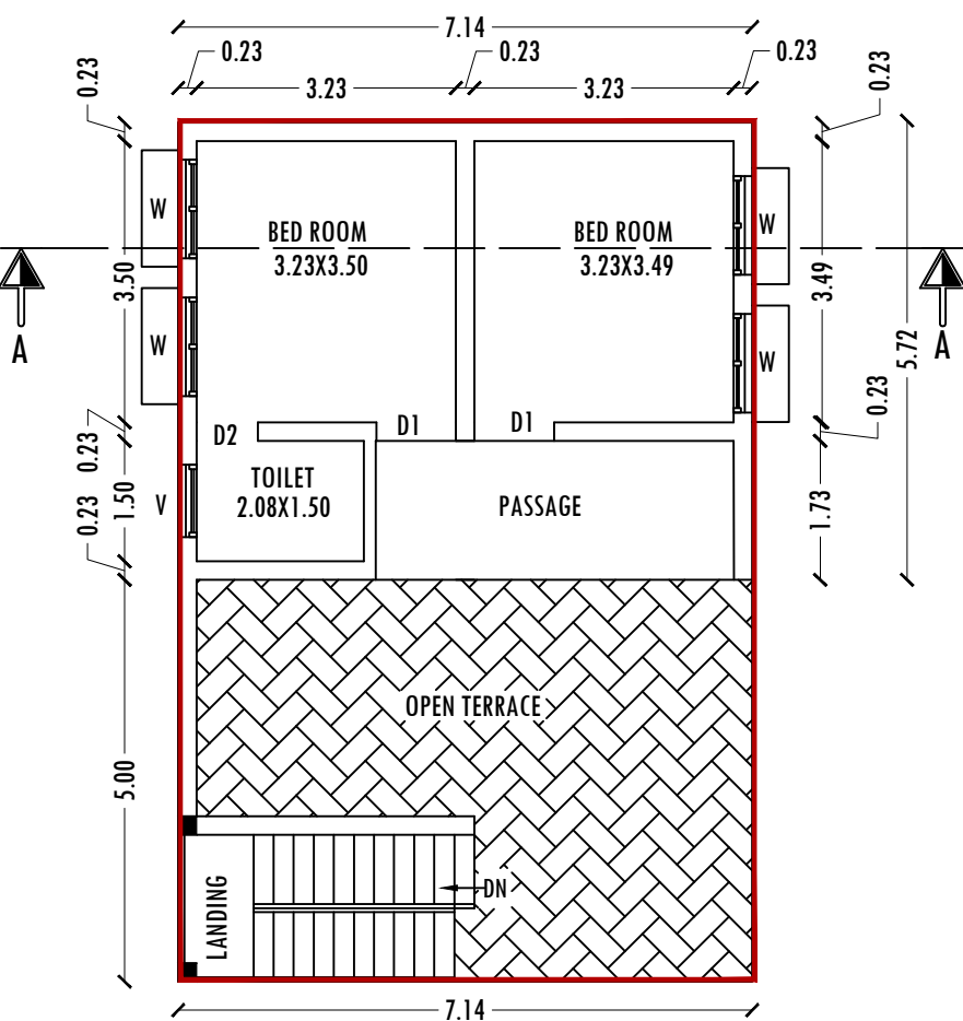
PRO-SECOND FLOOR PLAN
