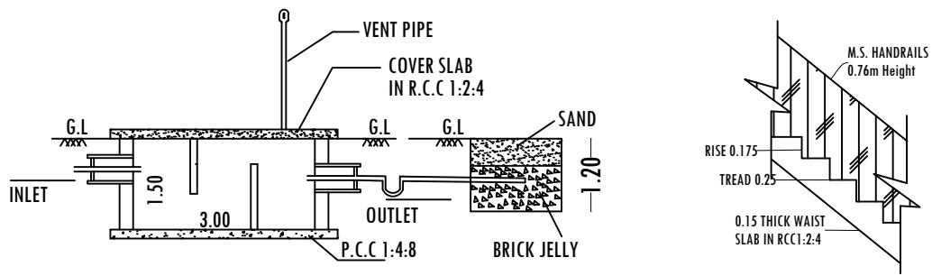
SECTION-AB
