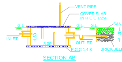
SECTION-AB
