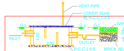
SECTION-AB
