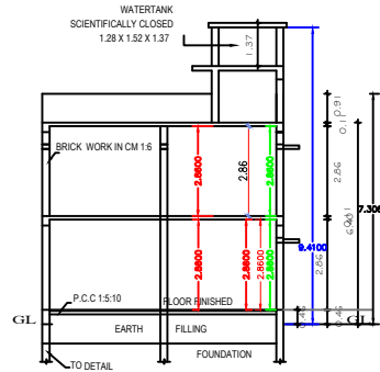
SECTION "A-B"
