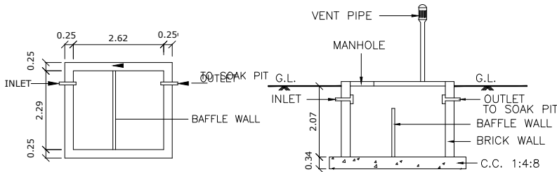
PLAN SEPTIC. TANK
