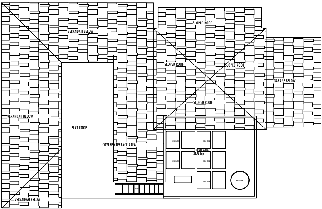
ROOF PLAN
