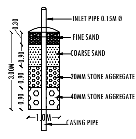
DETAILS OF RAIN WATER HARVESTING STRUCTURES
