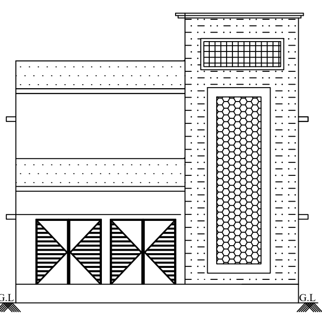
Elevation Plan
