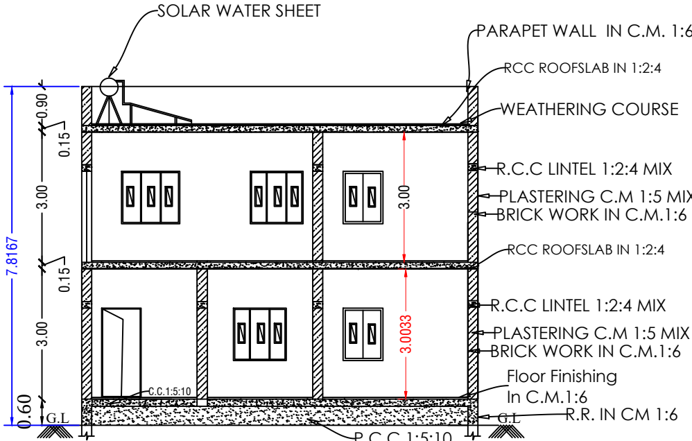
Section On-'AB'
