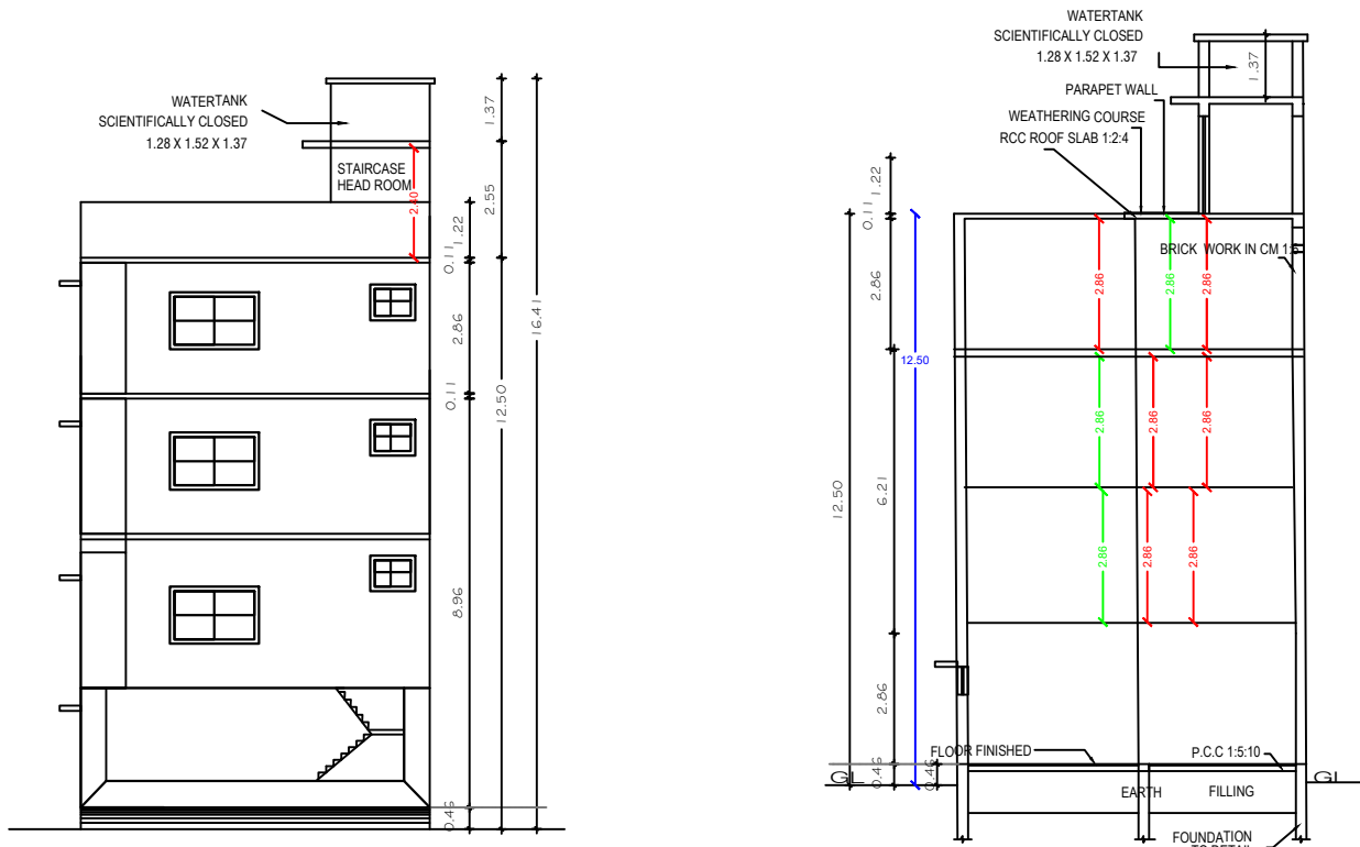
FRONT ELEVATION.
