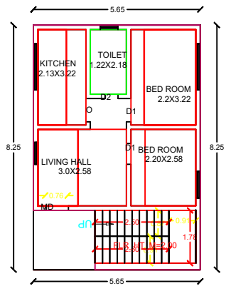
EXI.FIRST FLOOR PLAN.
