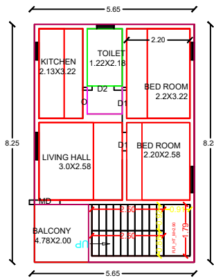
PRO. THIRD FLOOR PLAN.
