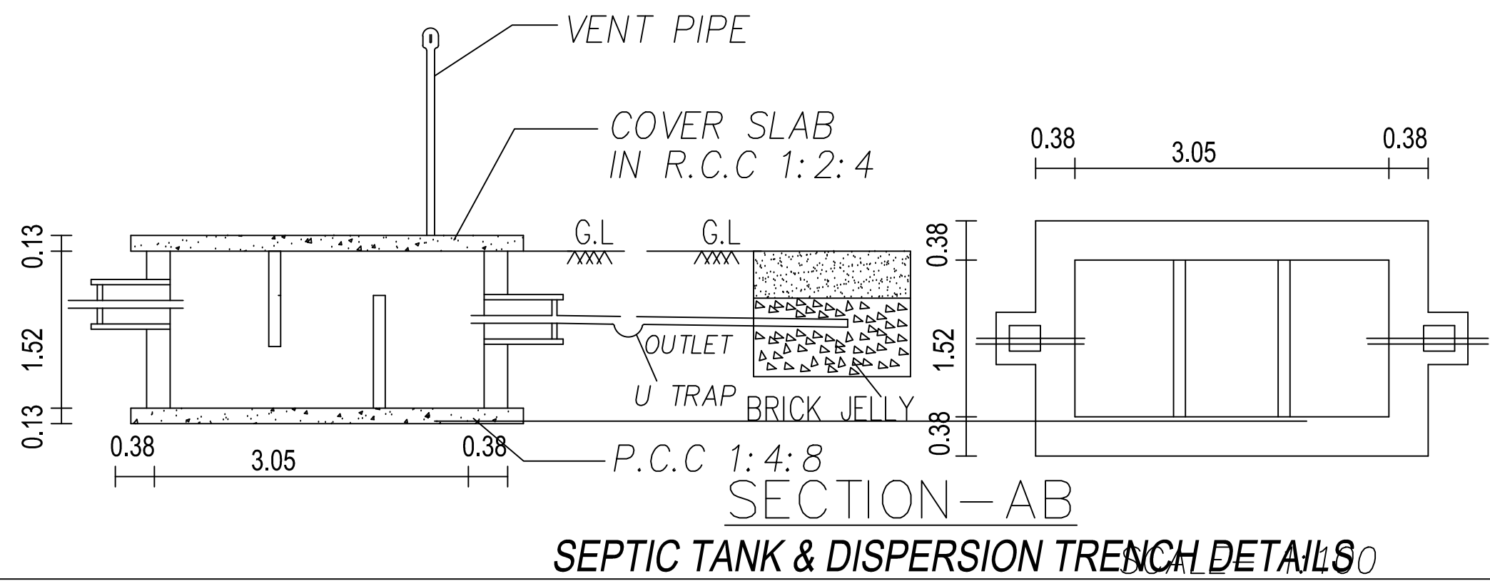
SEPTIC TANK & DISPERSION TRENCH DETAILS
