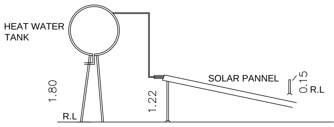
SOLAR WATER HEATER SYSTEM
