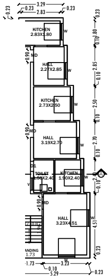
SECOND FLOOR PLAN SCALE:1:100
