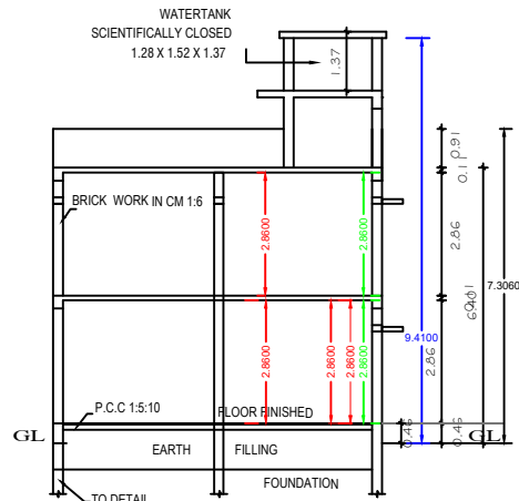
SECTION "A-B"
