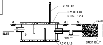
SECTION-A-B
