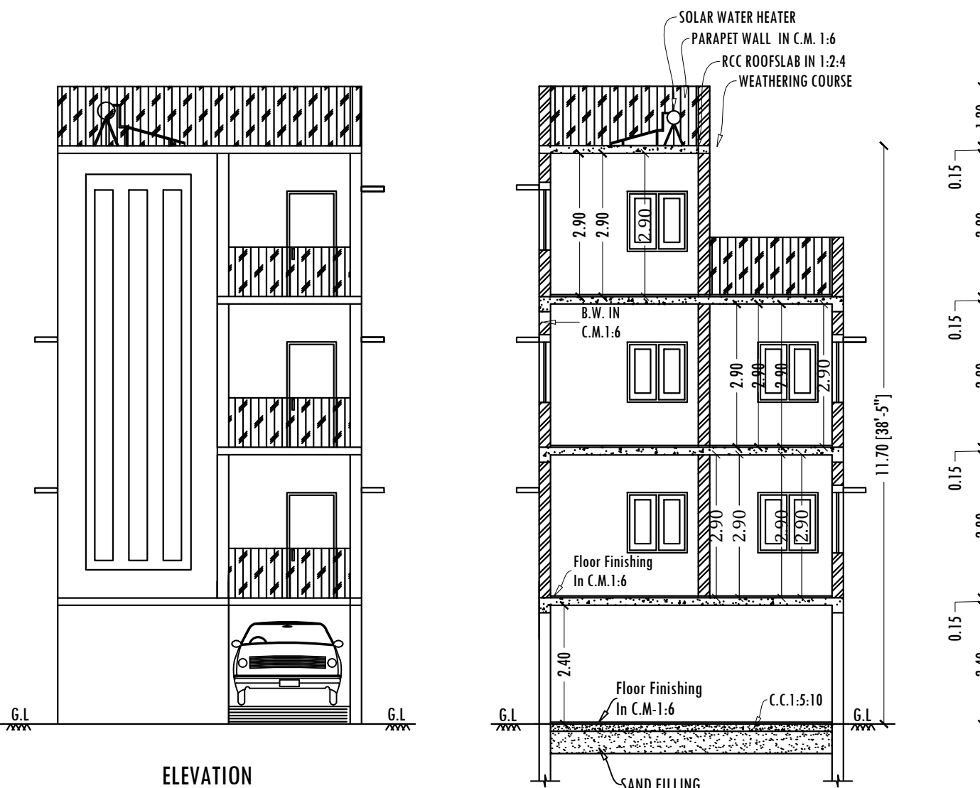
SECTION-AA
