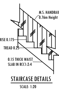
STAIRCASE DETAILS
