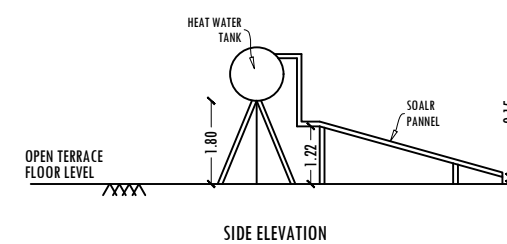
SIDE ELEVATION
