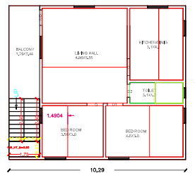
PRO. SECOND FLOOR PLAN.
