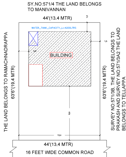
SITE PLAN
